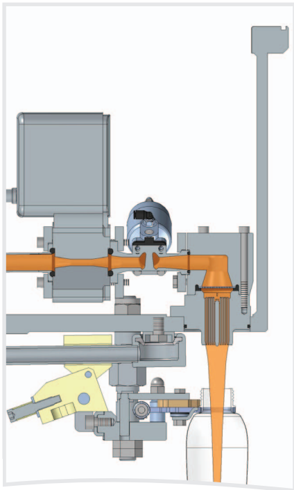
FX filling valve for still clear products
