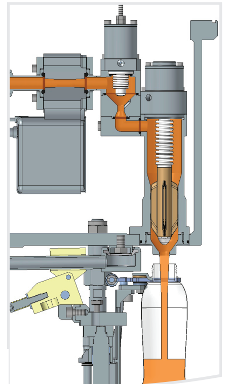
FX C filling valve for still products with and without pulps, fibres, pieces with dimensions up to 5x5x5 mm
