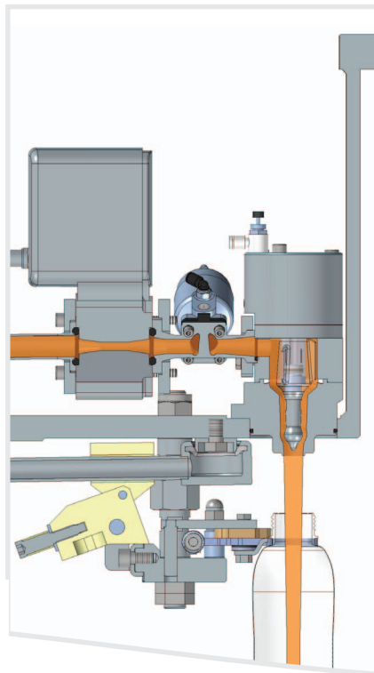
FX P filling valve for still products with and without pulps and fibres with maximum dimensions of 3 mm diameter x 20 mm length
